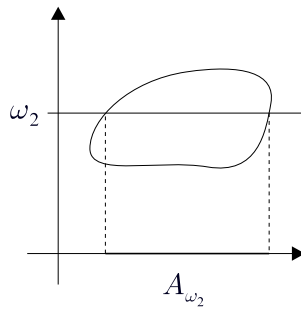
Figure 6.2 \omega_1 section of a set
